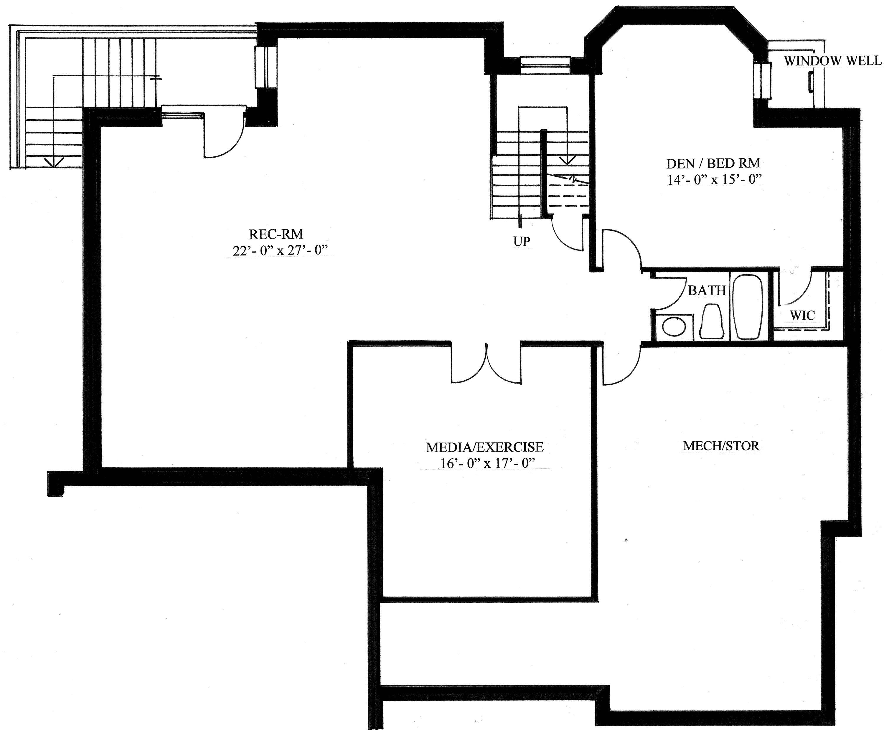
BASEMENT PLAN
