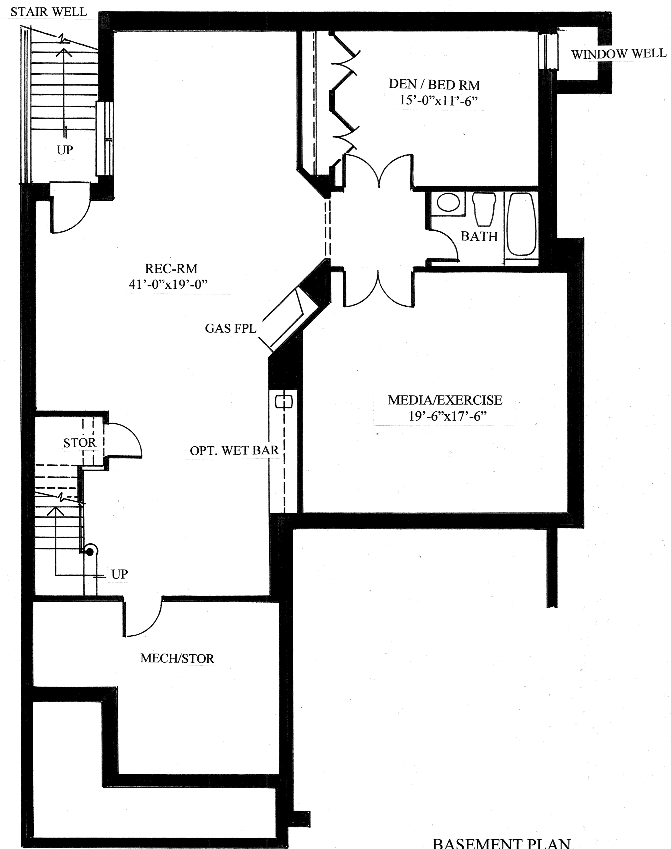
BASEMENT PLAN
