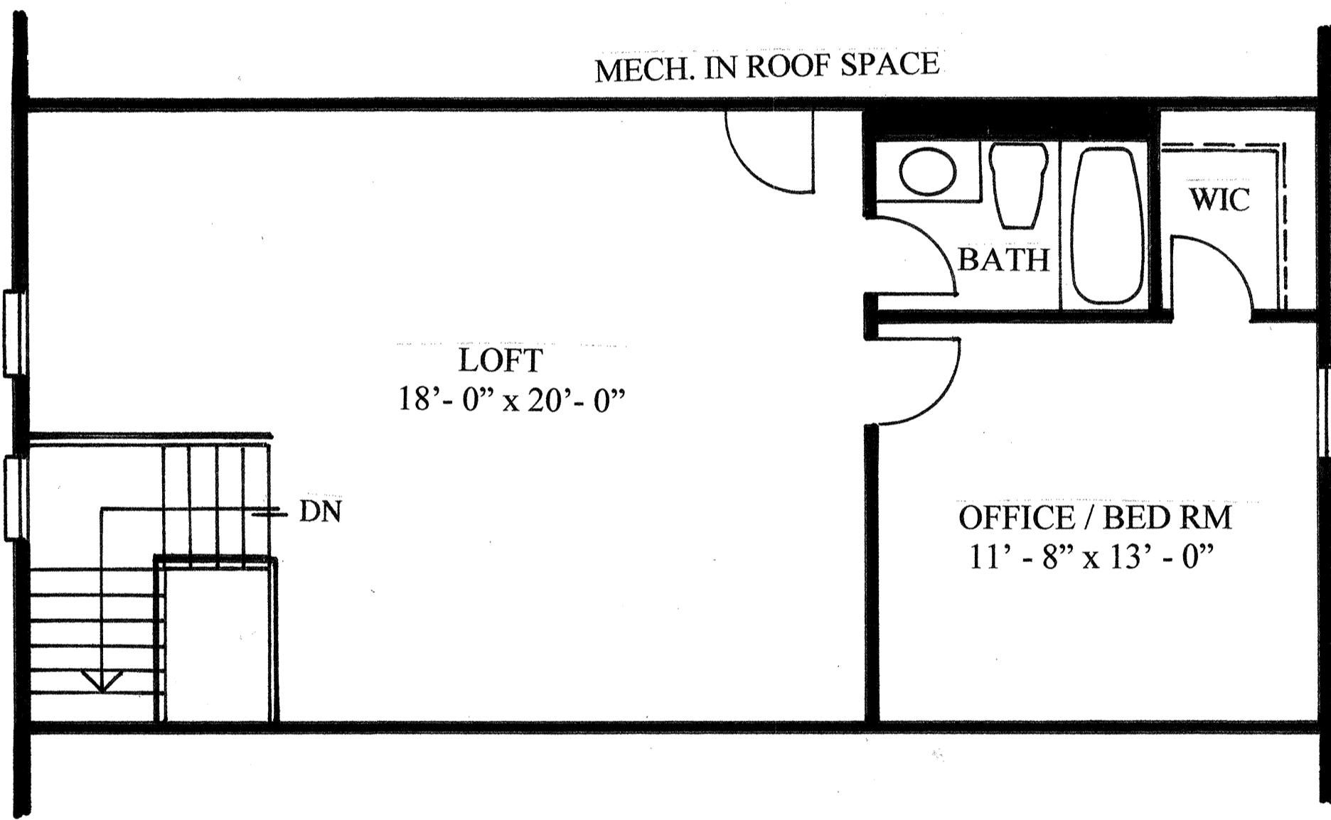
ATTIC PLAN
