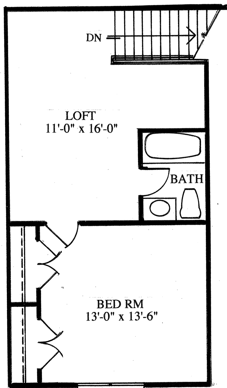
ATTIC PLAN
